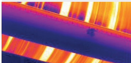
Monitoring drying stage in paper production.
